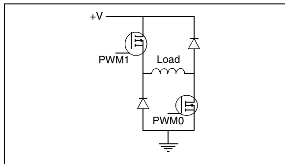
FIGURE 13-19: CENTER CONNECTED LOAD
