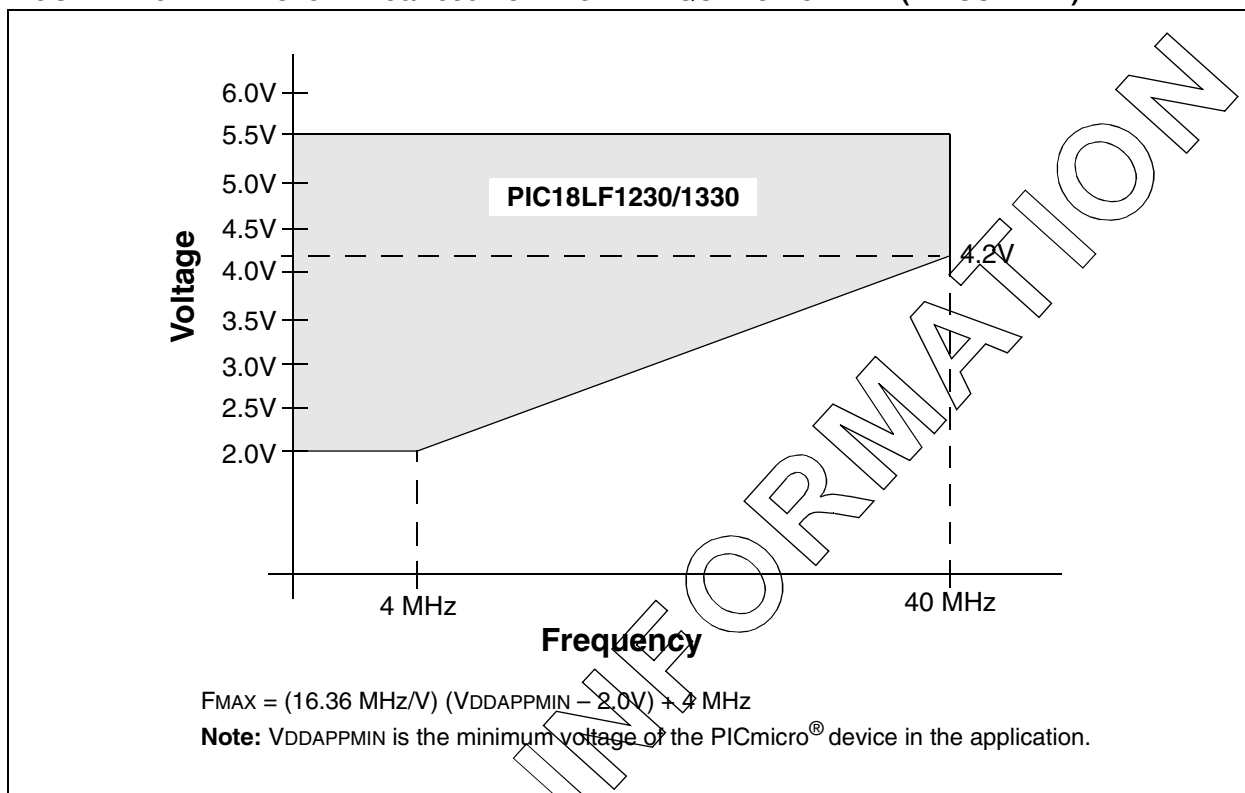
FIGURE 22-3: PIC18LF1230/1330 VOLTAGE-FREQUENCY GRAPH (INDUSTRIAL)
